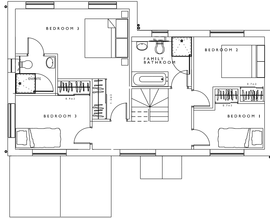
PROPOSED TYPICAL FIRST FLOOR PLAN 4 BEDROOM DWELLING PLOT 2
